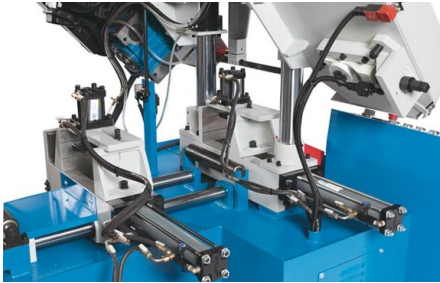
Bundle vise is provided for cutting entire material material to length
