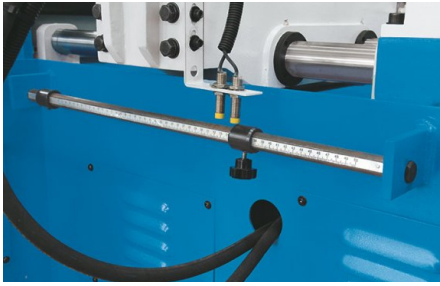
Automatic workpiece feed and traversing vise with manually adjustable stroke limit stop
